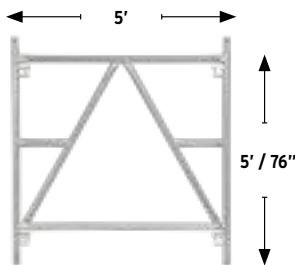
N HIGH LOAD CAPACITY FRAME 5' X 5' OR 5' X 76"
