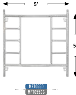
M DISMANTABLE FRAME
